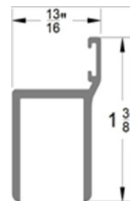
Semi-frameless Strike Cierre semi-enmarcado
